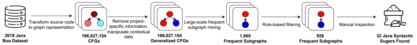
Figure 10: Overview of the workflow of our approach for discovering data-driven syntactic sugars
