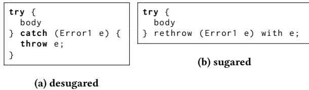
Figure 8: Potential syntax for Java rethrow
